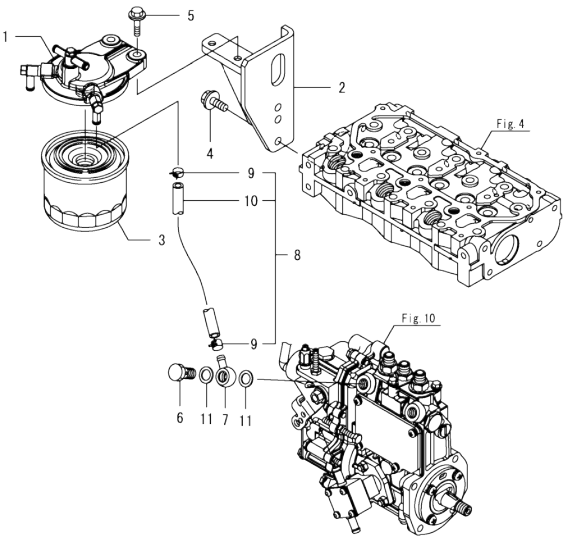
Fig.13. FUEL FILTER
